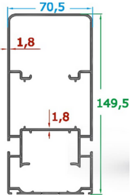
70'lik Eco Ray Profili/70 Eco Rail Profile
