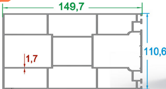
110'luk Eco Ray Profili/110 Eco Rail Profile
