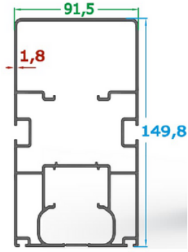
90'lik Eco Ray Profili/90 Eco Rail Profile
