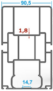
90'lik Ray Profili/90 Rail Profile
