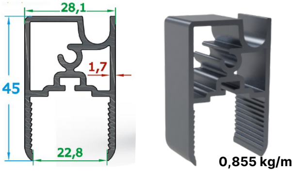
Alt Kanat Profili/Bottom Wing Profile
