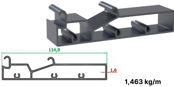
Baza Profili/Base Profile
