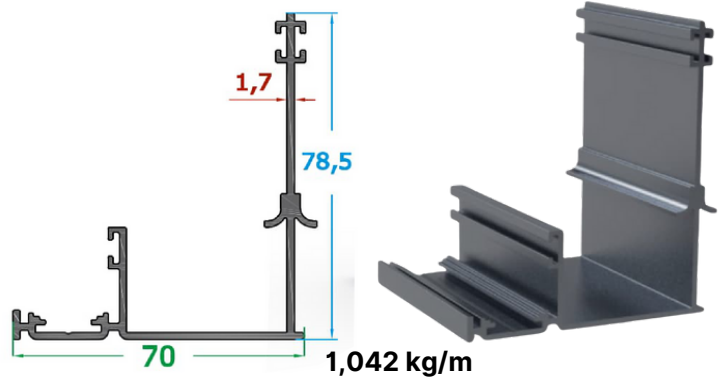
Alt Orta Yaprak Profili/Bottom Middle Leaf Profile
