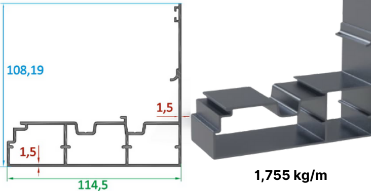
Ray Profili/Rail Profile
