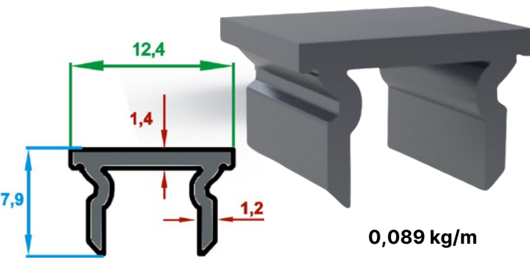
Yan Profil Kapak Profili/Side Profile Cover Profile
