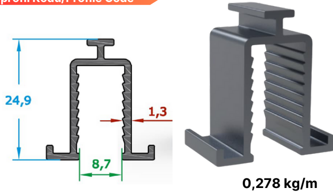
8mm Cam Profili/8mm Glass Profile
