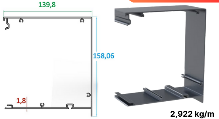
Motor Kutusu Profili/Engine Box Profile
