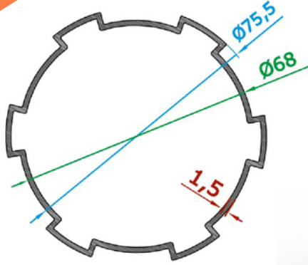
Motor Boru Profili/Engine Pipe Profile
