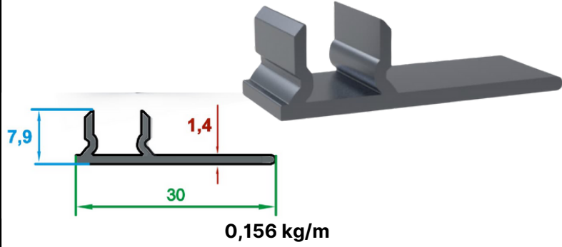
Alt Kasa Yan Kapak Profili/Bottom Frame Side Cover Profile
