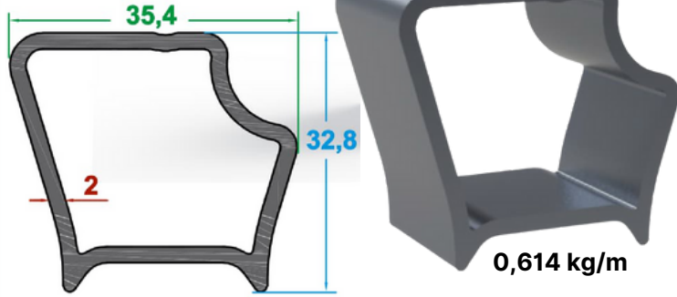
İnce Korniş Eki Profili/Thin Cornice Attachment Profile
