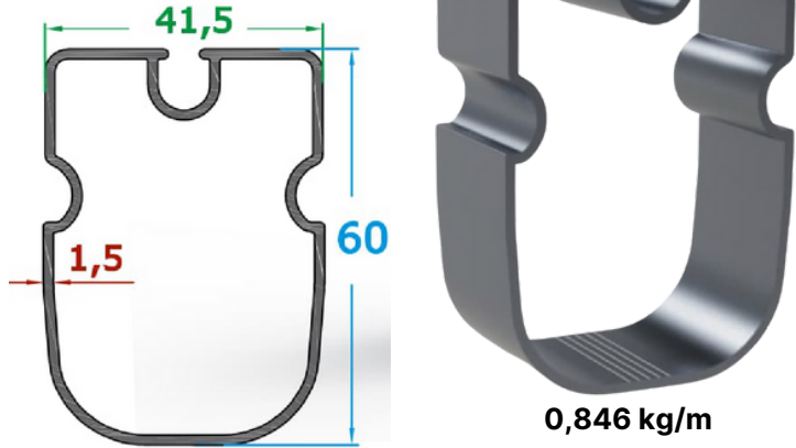
Damla İnce Korniş Profili/Drop Thin Cornice Profile
