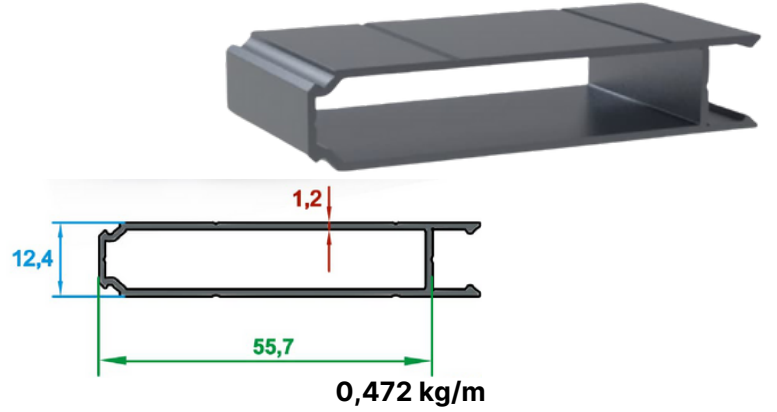
2'li Yan Profili/2 Side Profile
