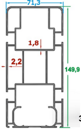
70'lik Ray Profili/70 Rail Profile
