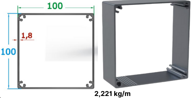
100x100 Dikme Profili/100x100 Strut Profile
