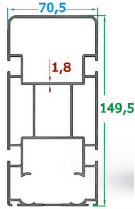
70'lik Orta Ray Profili/70 Medium Rail Profile
